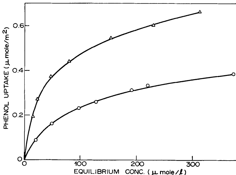
FIG. 4. Phenol adsorption isotherms from aqueous solution on Spheron-6 samples: ( \circ ) as-received; ( \triangle ) heat treated in \text{N}_2 at 600^\circ\text{C} .
