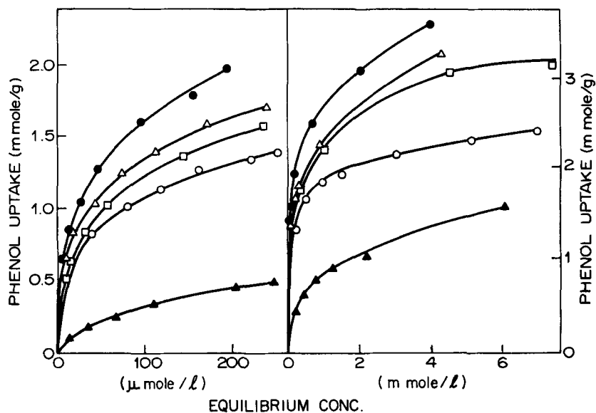
FIG. 3. Phenol adsorption isotherms from aqueous solution on various Saran carbon samples: (○) unactivated; (●) activated. Activated sample oxidized with: (△) \text{H}_2\text{O}_2 ; (□) (\text{NH}_4)_2\text{S}_2\text{O}_8 ; (▲) \text{HNO}_3 .
